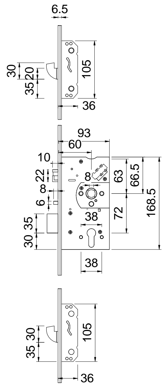
03 Front View 1 : 4
